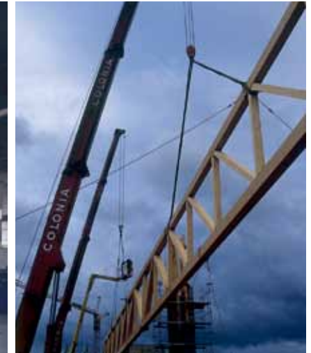
Aeroplane hangar, Köln-Bonn. architects Baugruppe Köln photographer Müller Blaustein
